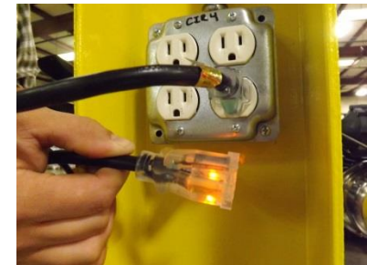
The extension cord has an illuminated female end that will easily identify that the heated PDU is operational. The installed heating control system will automatically activate when ambient temperatures are at 30° F or below.
